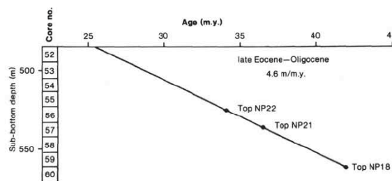
Figure 10. Magnetic polarity stratigraphy for the upper part of Hole 593.
