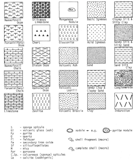
Figure 5. Standard symbols used to illustrate lithology.
