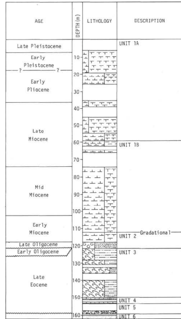
Figure 5. Stratigraphic sequence, Site 281 (Hole 281).
