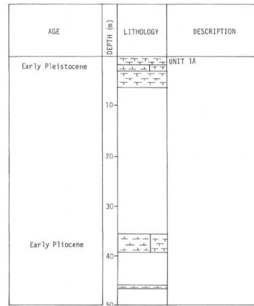
Figure 6. Stratigraphic sequence, Site 281 (Hole 281A).
