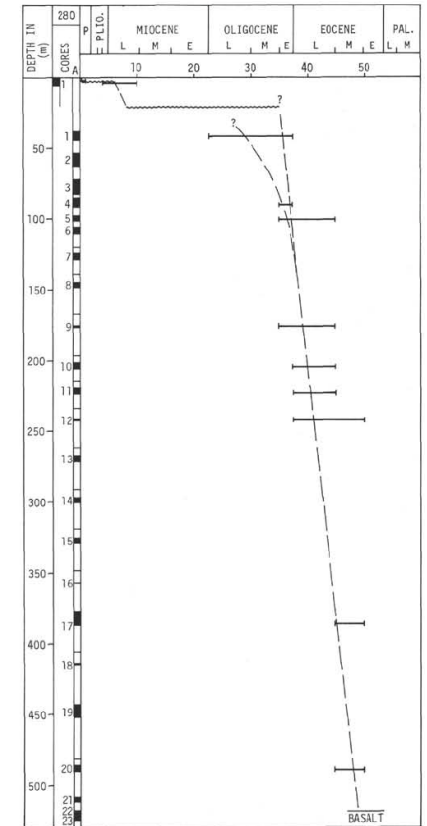
Age model :
