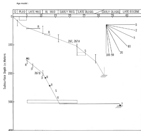
Figure 6. Comparison of accumulation rates between Holes 267-267A and Hole 267B.
