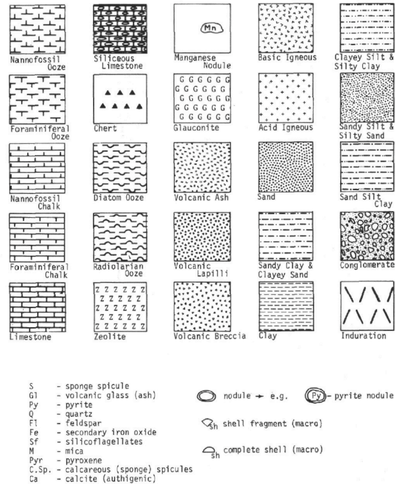
Figure 5. Standard symbols used to illustrate lithology.
