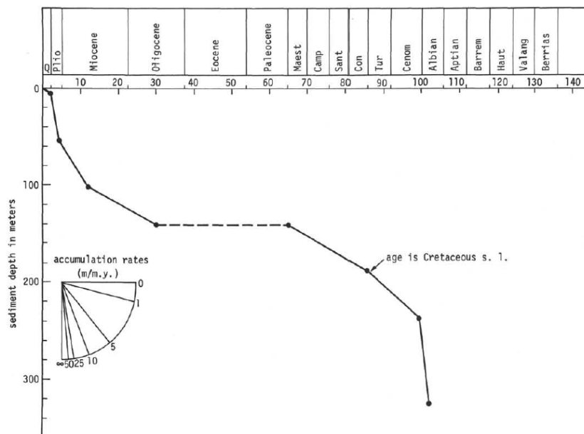
Figure 7. Sediment accumulation rates, Site 260.
