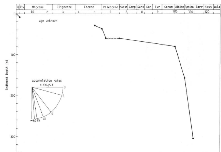
Figure 6. Sediment accumulation rates. Site 259.
