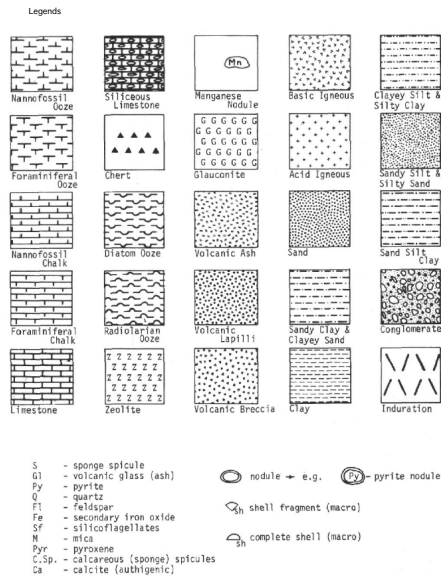
Figure 5. Standard symbols used to illustrate lithology.
