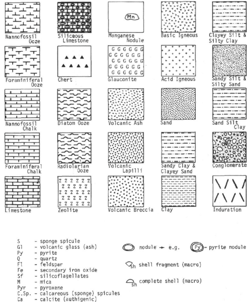
Figure 5. Standard symbols used to illustrate lithology.
