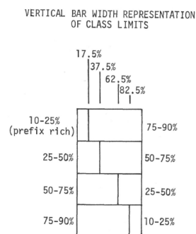
Figure 6. Vertical bar width representation of class limits.
