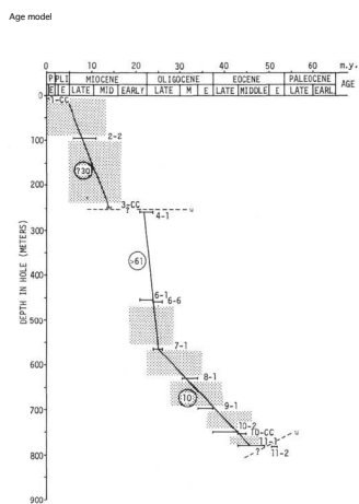
Figure 4. Sedimentation Rate Curve, Site 224. Plotted bars are those sufficient to control slopes of lines. Stippled pattern represents some uncored intervals. See Chapter 2,
