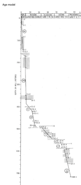
Figure 6. Sedimentation Rate Curve, Site 223. Plotted bars are those sufficient to control slopes of lines. Stippled pattern represents some uncored intervals. See Chapter
