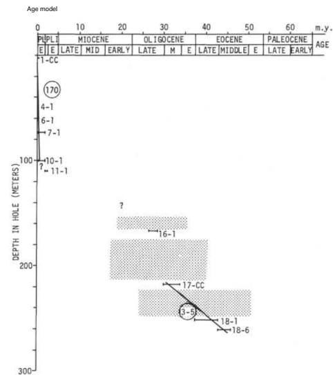
Figure 7. Sedimentation Rate Curve, Site 221. Plotted bars are those sufficient to control slopes of lines. Stippled pattern represents some uncored intervals. See Chapter
