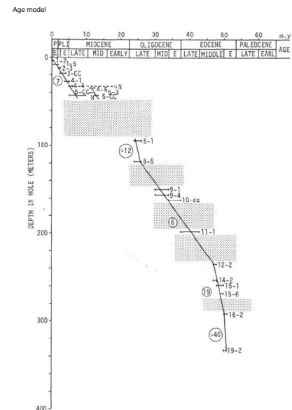
Figure 6. Sedimentation rate curve, Site 220. Plotted bars are those sufficient to control slopes of lines. Stippled pattern represents some uncored intervals. See Chapter 6.
