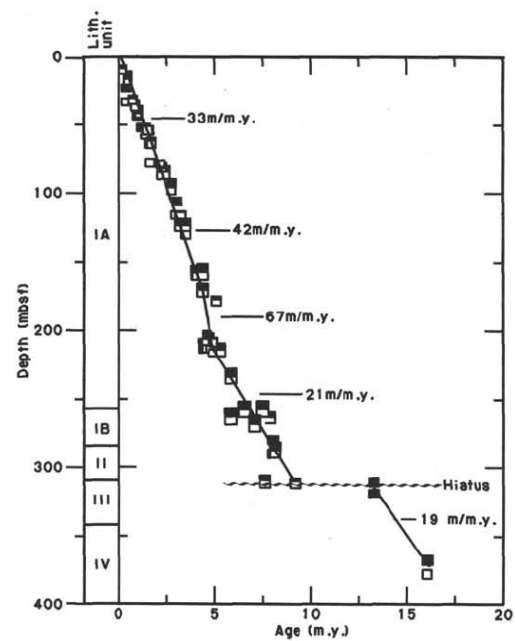
Age model:
