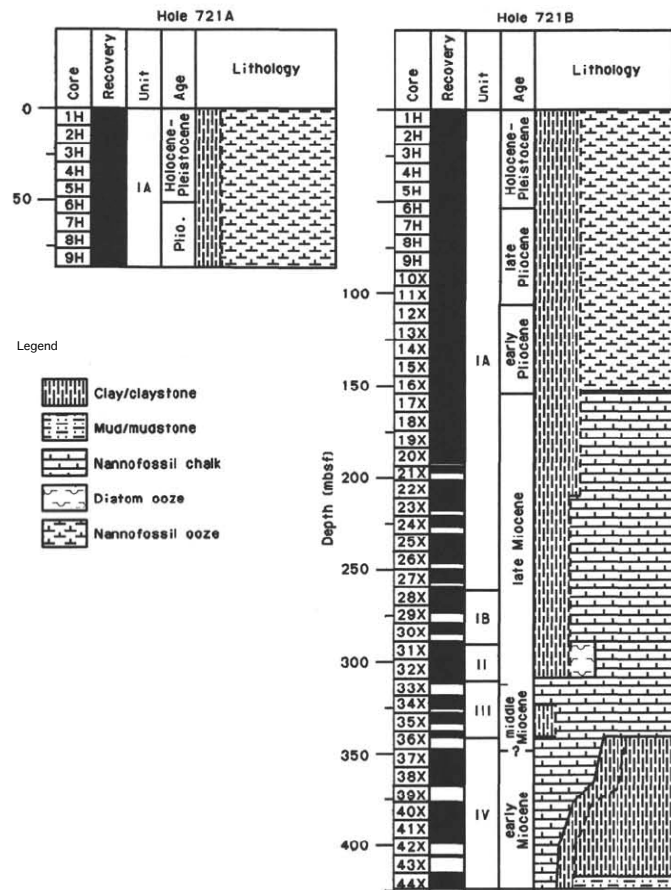
Age model:
