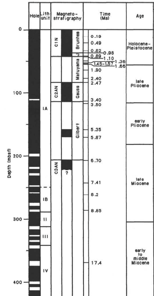
Magnetostratigraphy
