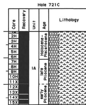
Age model:
