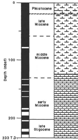
Figure 2. Stratigraphic summary, Site 714. Black column represents recovered section.
