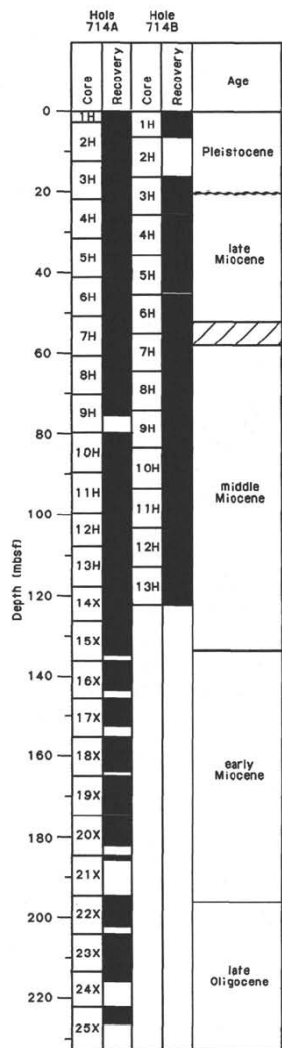
Figure 2. Stratigraphic summary, Site 714. Black column represents recovered section.
