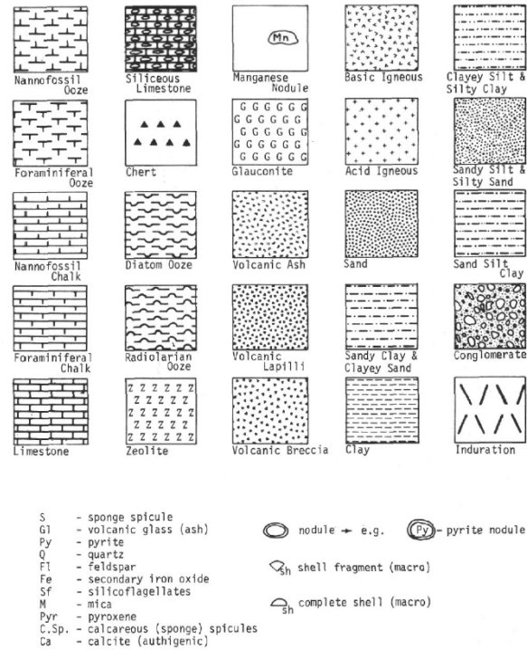
Figure 5. Standard symbols used to illustrate lithology.
