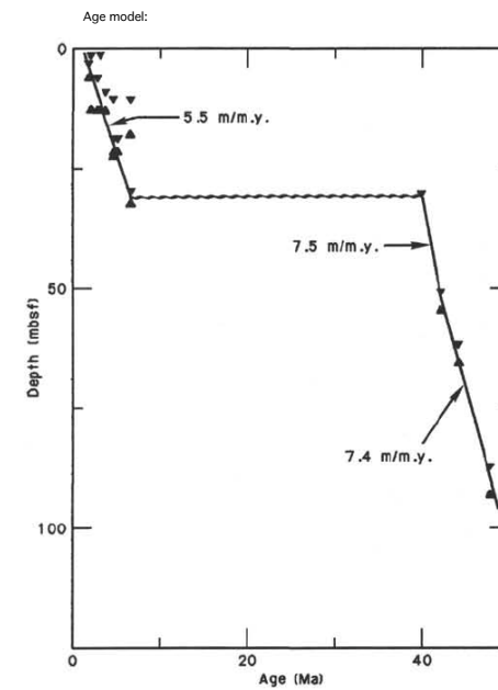
Figure 16. Sedimentation rates at Site 713 based on biostratigraphic datums listed in Table 4.
