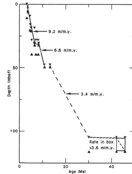
Figure 15. Sedimentation rates at Site 712 based on biostratigraphic datums listed in Table 3.
