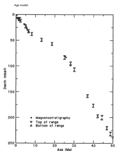
Figure 13. Age-depth plot for Hole 711A based on nannofossil datum events and magnetic reversal boundaries.
