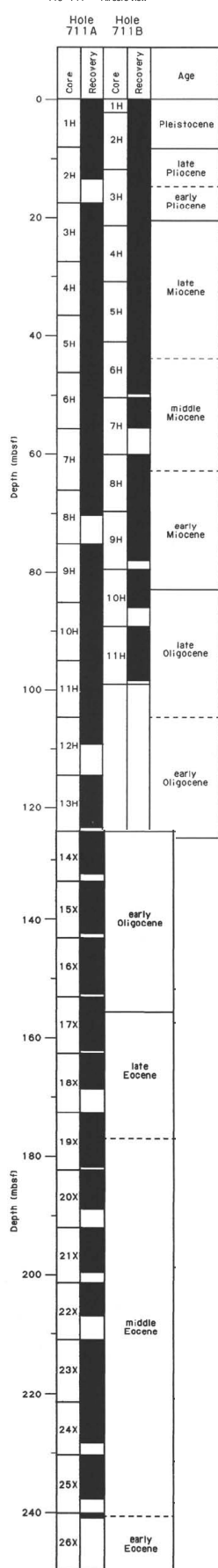
Figure 2. Stratigraphic summary of Site 711. Black column represents recovered section.
