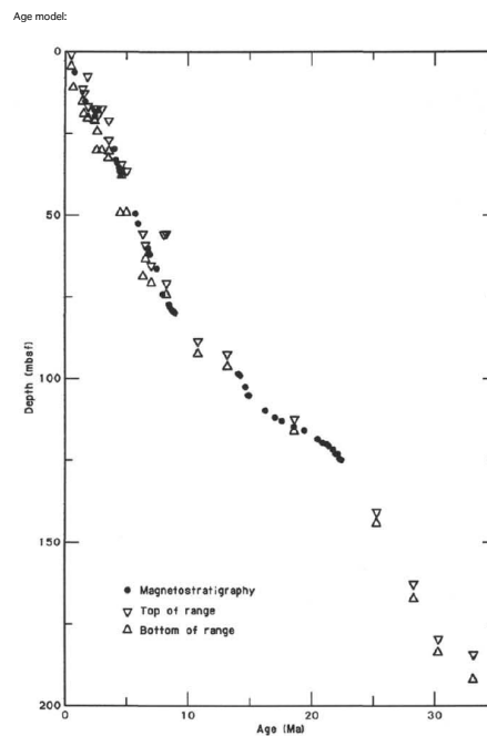
Figure 16. Sedimentation rates in Hole 710A based on the biostratigraphic datum levels listed in Table 3. Age-depth relationships for magnetostratigraphic reversal boundaries are listed in Table 2.
