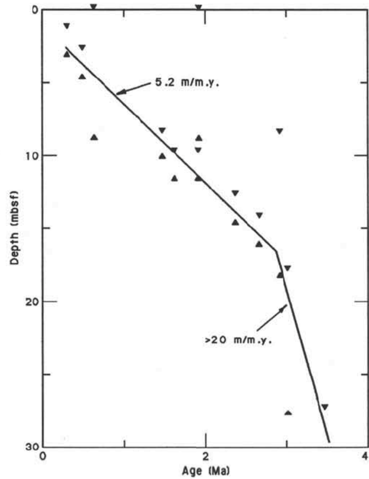
Figure 24. Sedimentation-rate curve for Hole 705A.
