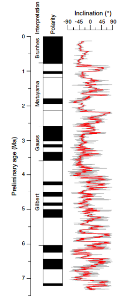
Figure F27. Spliced inclination record, Site U1476. Age based on a preliminary shipboard age model. Gray line indicates the inclination after 15 or 25 mT demagnetization, red line corresponds to 15-point running average. Polarity chron ages after Gradstein et al. (2012).
