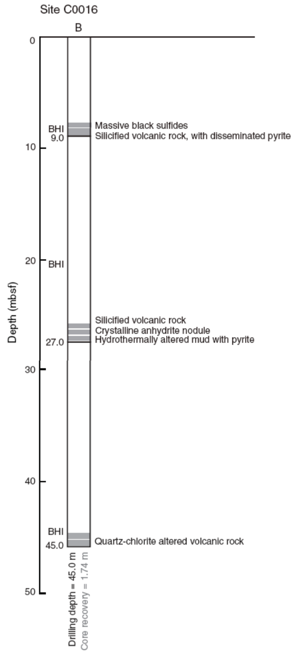
Figure F13. Schematic illustration of drilling and coring systems used, drilling and core recovery depths, and brief remarks on drilling operations and specific features of cores recovered from Site C0016. NBC = North Big Chimney. BHI = Baker-Hughes Inteq.
