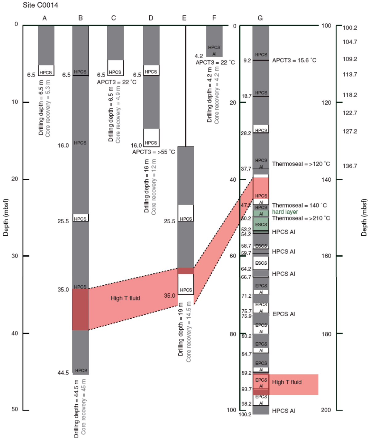
Figure F10. Schematic illustration of drilling and coring systems used, drilling and core recovery depths, and brief remarks on drilling operations and specific features of core recovered from Site C0014. High T = high-temperature.
