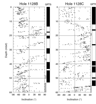
Magnetostratigraphy
