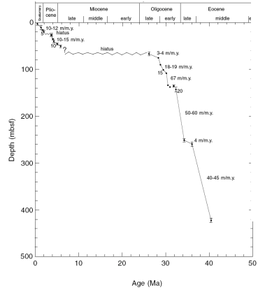
Age model
