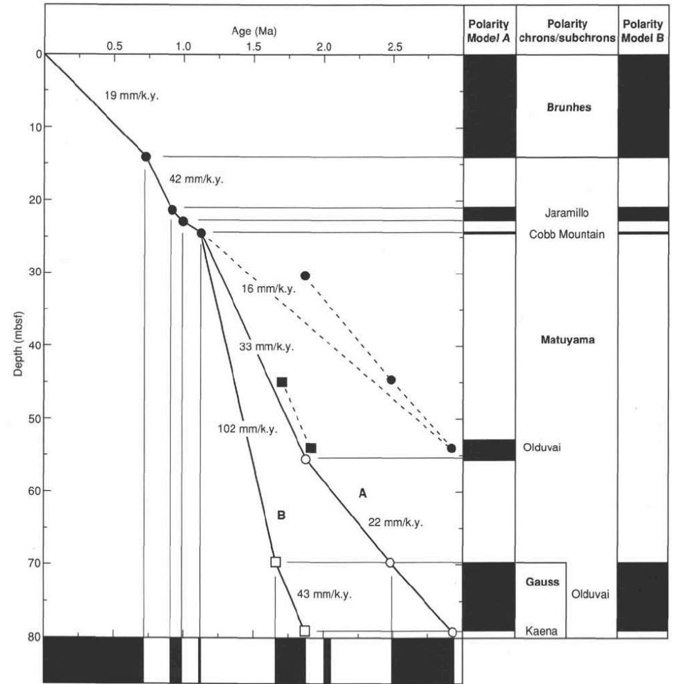
Polarity model
