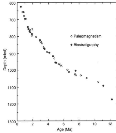
Age model
