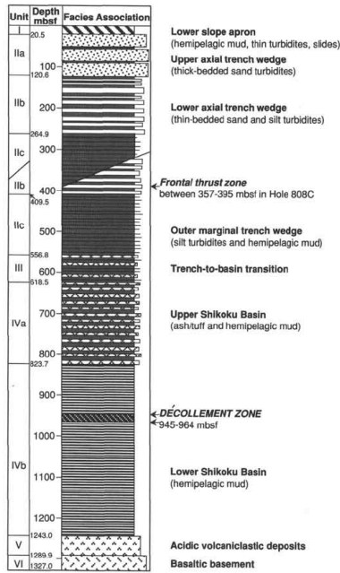
Lithology
