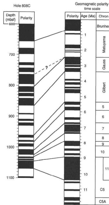
Magnetostratigraphy
