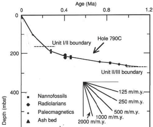
Age model
