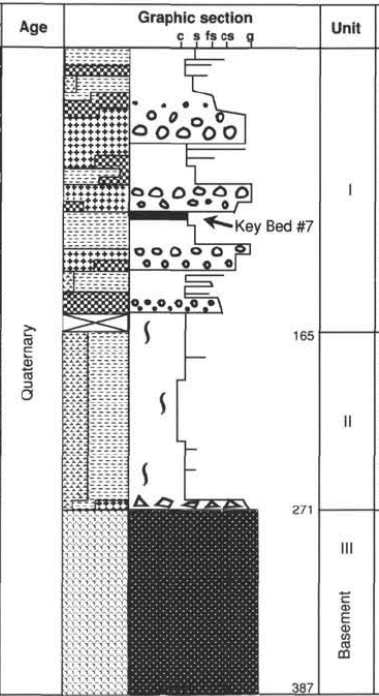
Lithology
