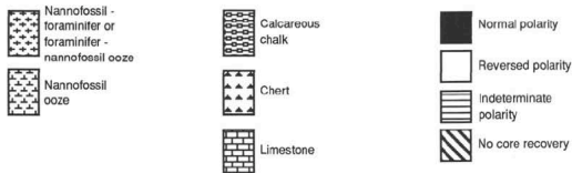
Key to lithology and magnetic polarity
