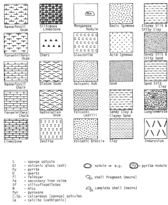
Figure 5. Standard symbols used to illustrate lithology.
