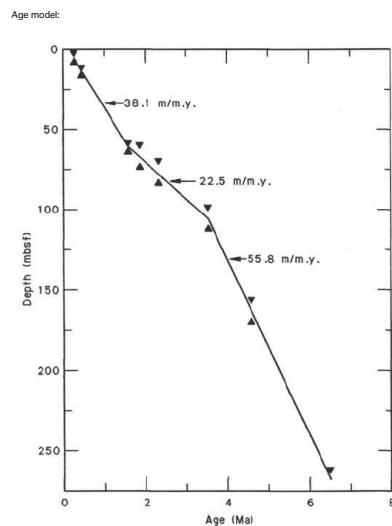
Figure 6. Sedimentation rates computed for Hole 716B using nannofossil datum levels discussed in text.
